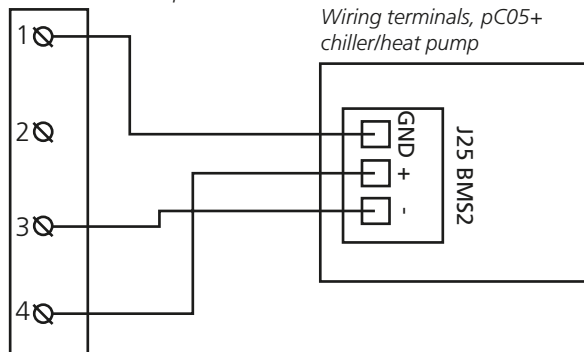
Wiring terminals for the TBLZ-64 cable adapter
